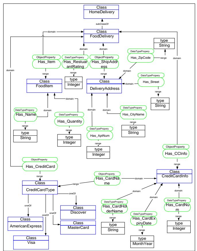
Figure 1: Domain Ontology for Home Delivery of Food
