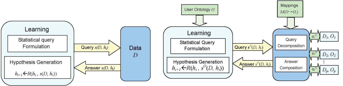
Figure 1: (Left) Learning = Statistical Query Answering + Hypothesis Generation (Right) General Framework for learning classifiers from semantically heterogeneous distributed data.
