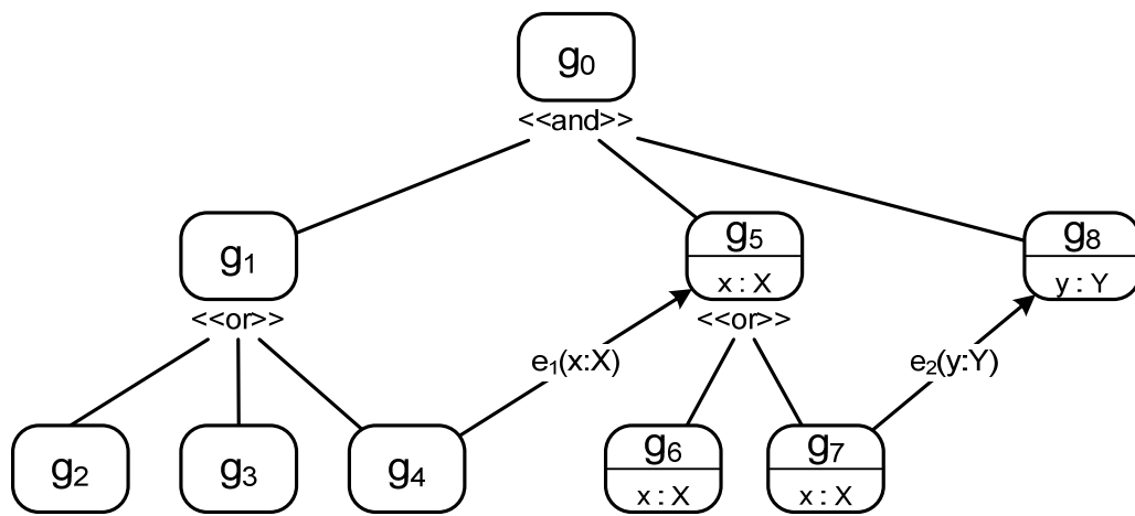
Figure 1. Goal specification tree
