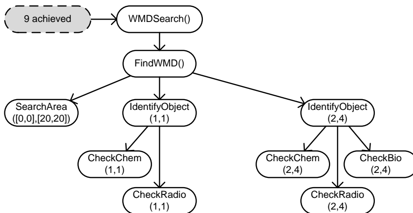
Figure 11. CheckBio(1,1) is achieved
